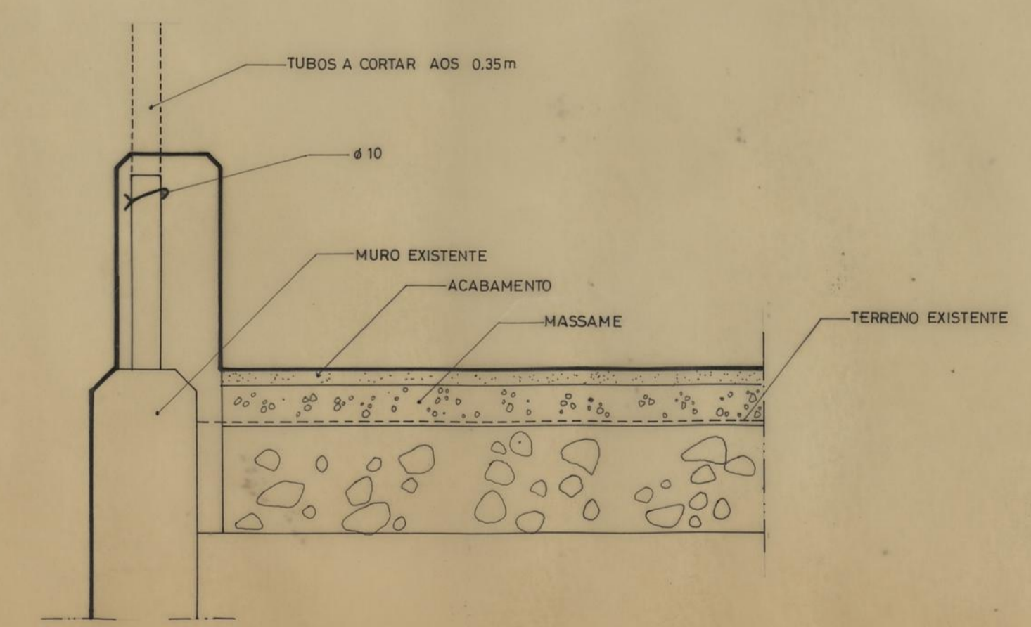
PORMENOR A
